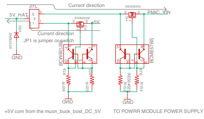
Circuit 1
