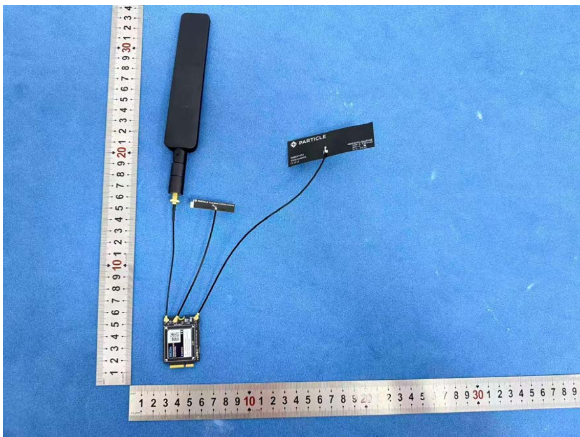
Photo 4 - External view of EUT
