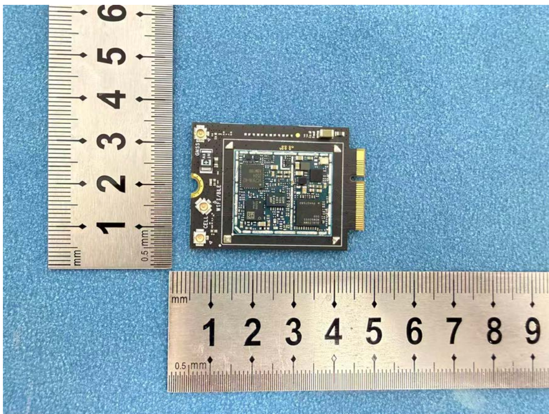
Photo 5 - Internal view of EUT
