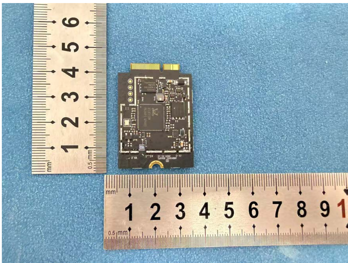
Photo 6 - Internal view of EUT
