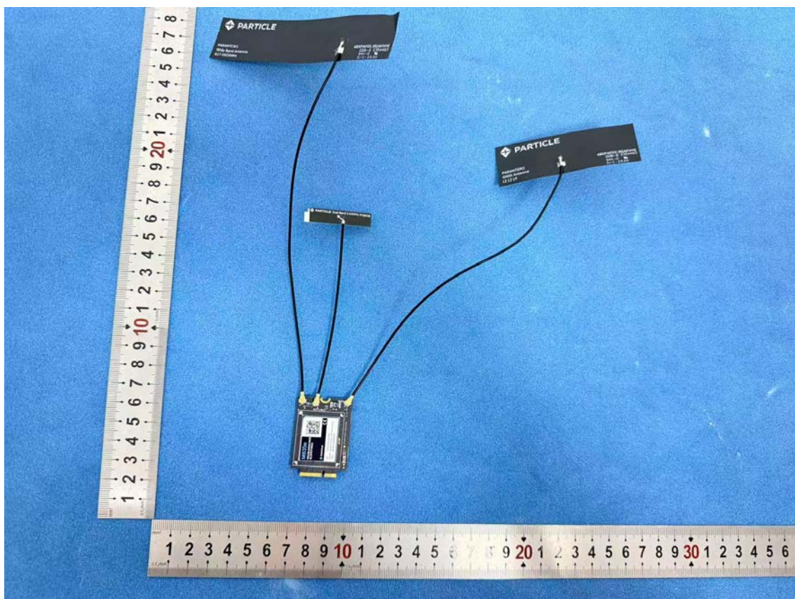
Photo 3 - External view of EUT
